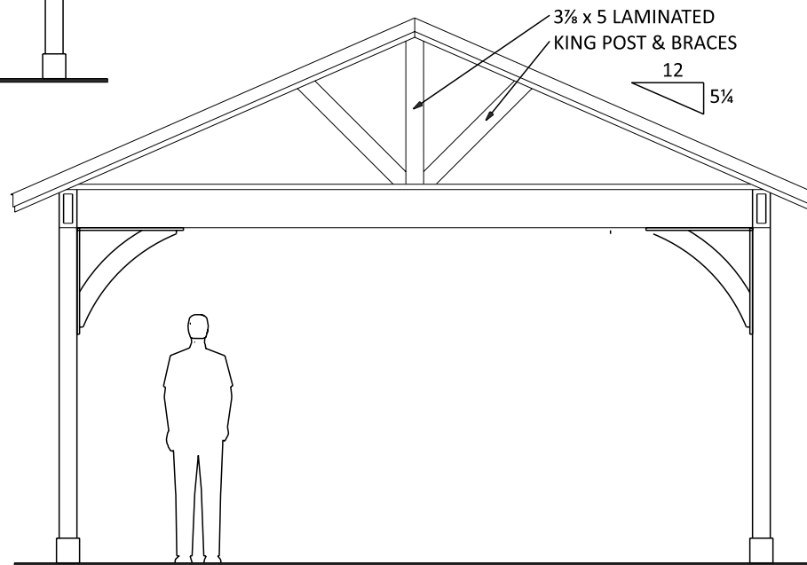
Side Elevations
