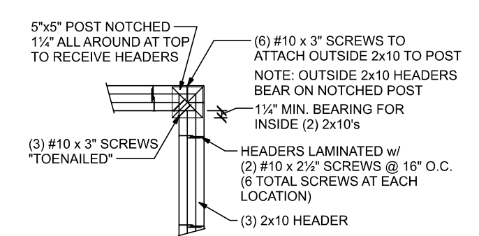
HEADER TO POST CONNECTION DETAIL SCALE: 1/2" = 1'-0"
