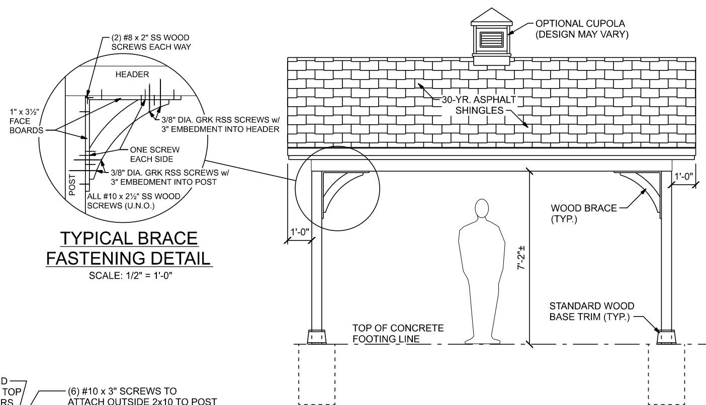
SIDE ELEVATION
