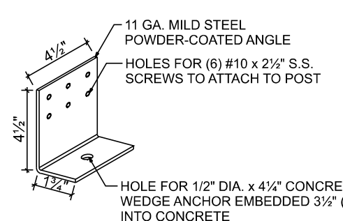
STEEL L-BRACKET DETAIL NO SCALE
