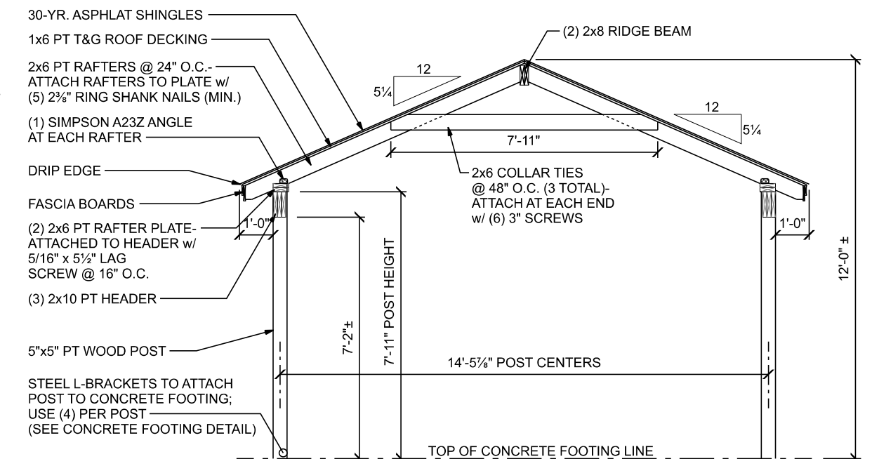
CROSS SECTION
