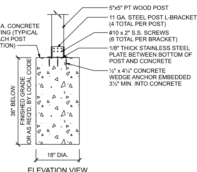
CONCRETE FOOTING DETAIL SCALE: 1/2" = 1'-0"
