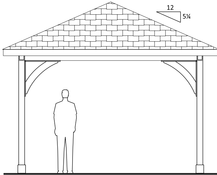
Front Elevation
